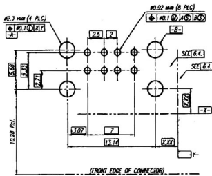
FIGURE A: PCB FOOTPRINT FOR RECEPTACLE, (THROUGH-HOLE)
